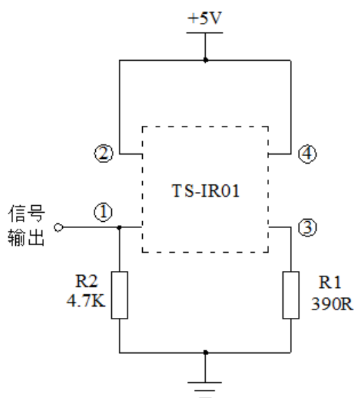
DC 5V 典型应用电路, DC 5V Typical application circuit
