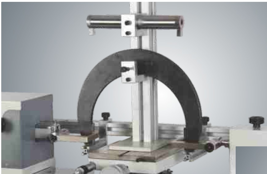
Snap Gauge C Type (above 300 mm) measurement : Hold on universal holder
