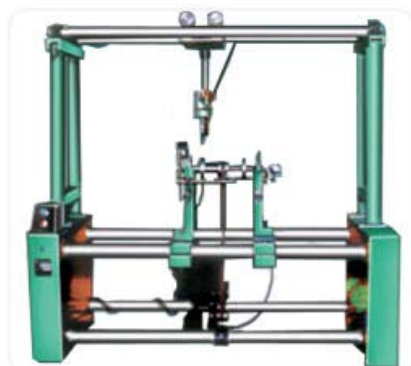
Machine provided with optional vertical drilling attachment
