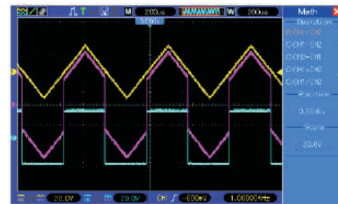
Math: CH1+CH2
