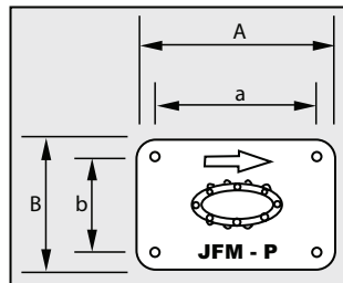
External Mounting Plate
