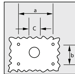
Probe Insertion Cut-out
