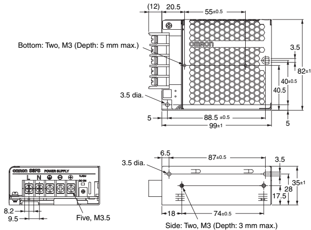
Panel mounting hole dimensions
