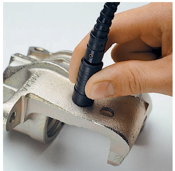
Measuring on rough surfaces, Zn/Fe with the ESD20Zn probe
