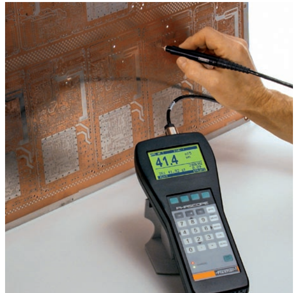
Measuring copper thickness in through-holes using the ESL080B probe
