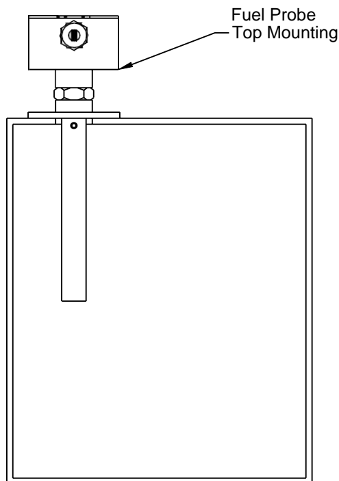
Figure 2 : Mounting Arrangement
