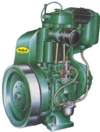
5 HP to 10 HP Single Cylinder, Water Cooled & Air Cooled, Tapper Roller Bearing (TRB) and Bush Bearing (BB) type, High Speed Diesel Engine Couple Sets
