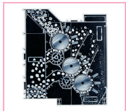
CROSS SECTION SUPER III STICK MACHINE
