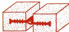
Top position of multi ribbed central bulb type of P.V.C. Water Stop after differential settlement
