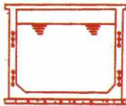
P.V.C. Water stop in R.C.C. Water tank
