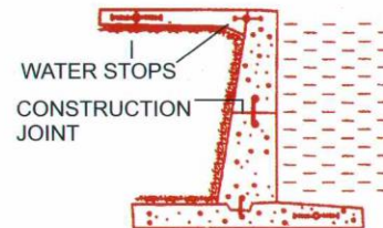
Construction Joint Water Reservoir Swimming Pool etc.
