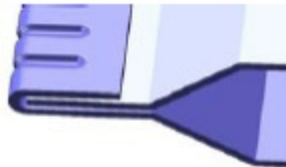
Single folded edge @3 times plate thickness
