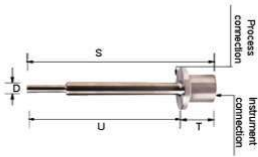
BAR STOCK REDUCED TIP VAN STONE THERMOWELL
