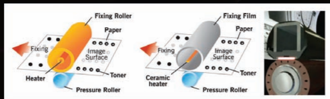
Traditional Roller Fixing
